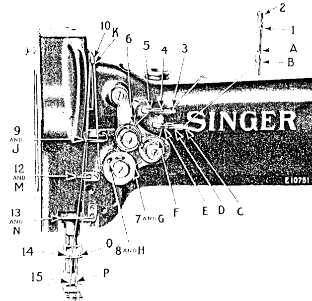
Fig. 13. Upper Threading
